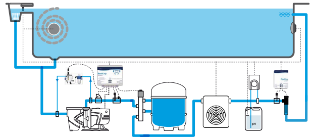
INSTALLATION TYPIQUE ELECTROLYSE
